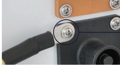
Step 9: Fix one end of the grounding cable, then reattach the screw over the top, securing the cable.
