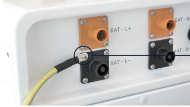
Step 8: Loosen this specific screw.
