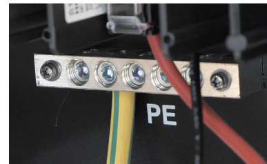
Step 10: Connect the grounding cable to the inverter's PE.
